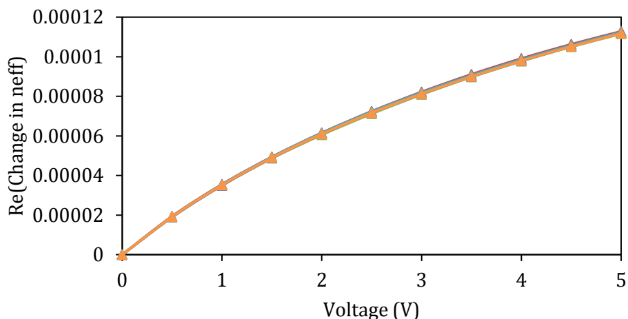
Figure 12. Change in effective index versus voltage applied. (Dark blue line: 200nm waveguide height; Orange line: 220nm waveguide height; Grey line: 240nm waveguide height; Yellow line: 260nm waveguide height; Light blue line: 280nm waveguide height; Green line: 300nm waveguide height).
