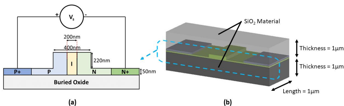
Figure 1. (a) Shows the cross section of the waveguide; (b) Shows the waveguide block structure.
